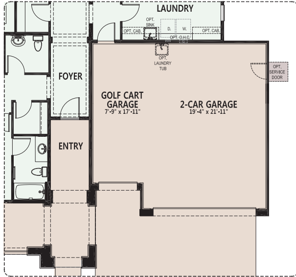
Opt.4 ft Garage Extension Elevation 'D'
